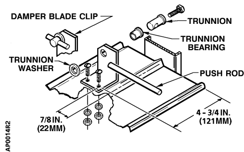
Figure 4. Damper Blade Clip Kit 331-838.
