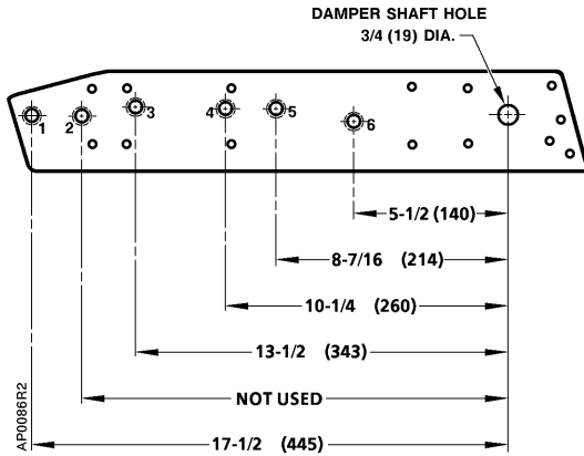
Figure 12. Actuator Mounting Plate 331-623 Pivot Shaft Locations. Dimensions in Inches (Millimeters).
