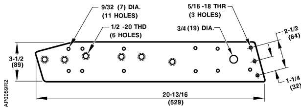
Figure 15. Actuator Mounting Plate 331-623. Dimensions in Inches (Millimeters).
