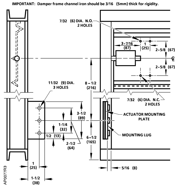
Figure 9. Frame Mounting—Type B. Dimensions in Inches (Millimeters).
