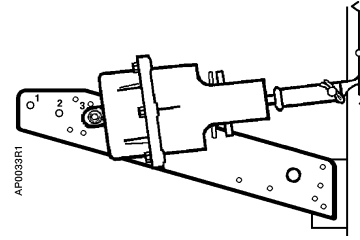
Figure 11. Frame Mounting, Normally Closed Damper.
