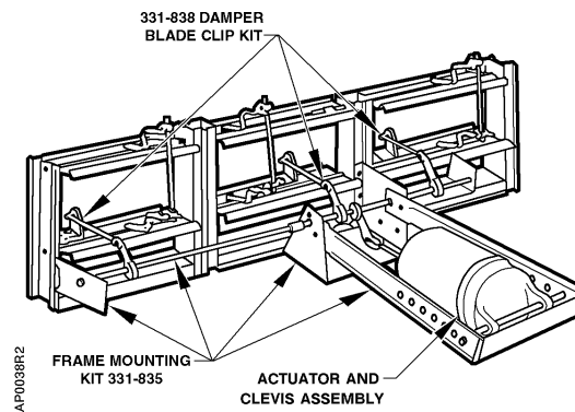
Figure 8. Three-Section Damper.
