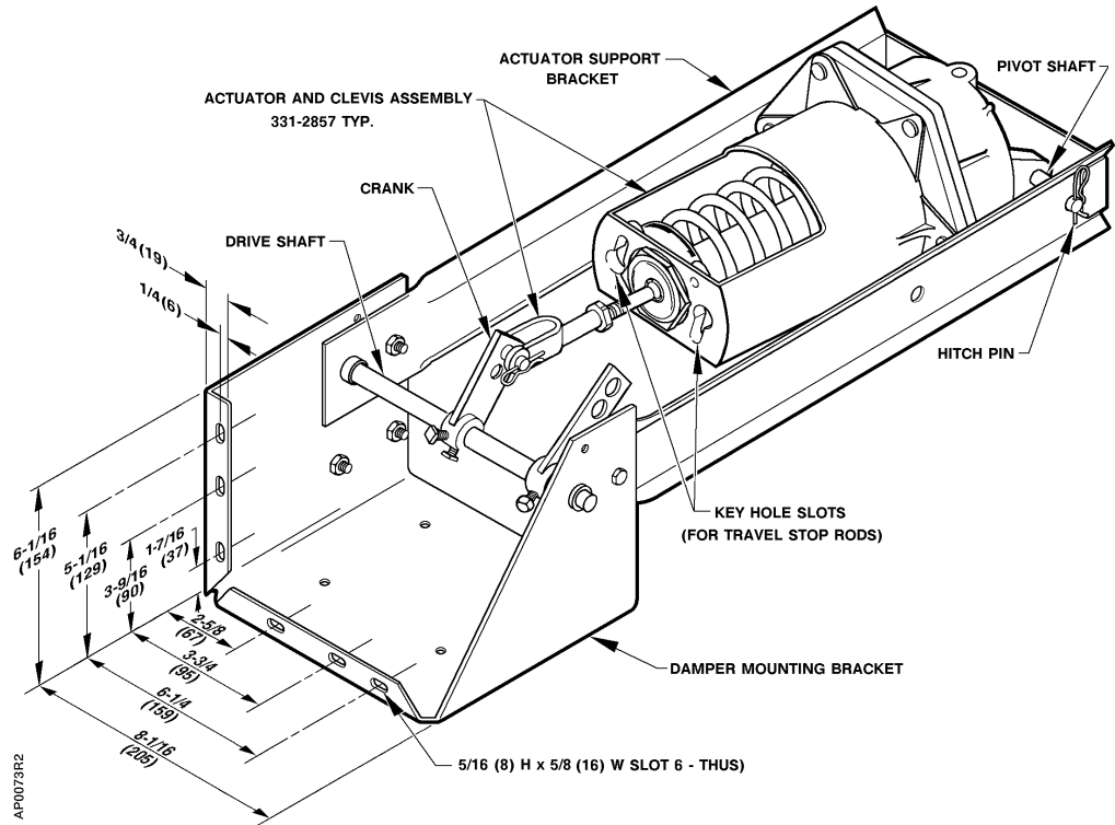
Figure 7. Actuator and Clevis Assembly 331-2857 (Typical) Attached to Frame Mounting Kit 331-833. Dimensions in Inches (Millimeters).
