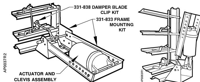
Figure 5. One-Section Damper.
