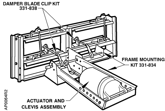
Figure 6. Two-Section Damper.
