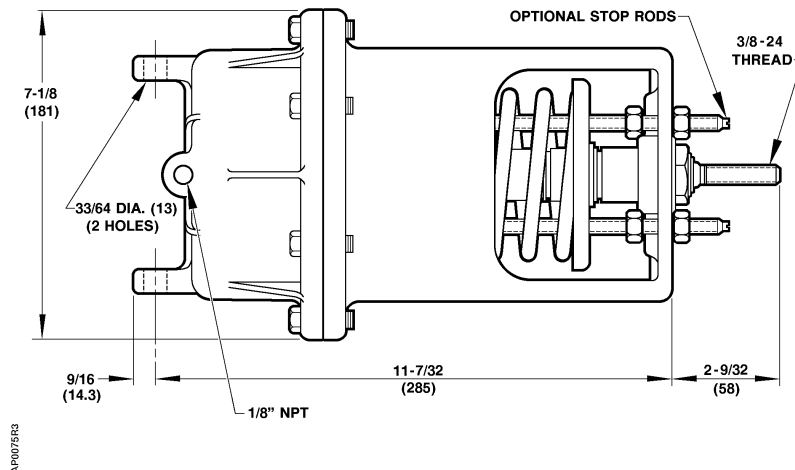
Figure 13. Extended Shaft Remote Mounting with Travel Stops. Dimensions in Inches (Millimeters).
