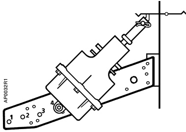
Figure 10. Frame Mounting, Normally Open Damper.
