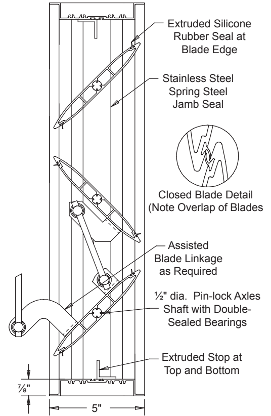
A29 (Opposed Blade)
