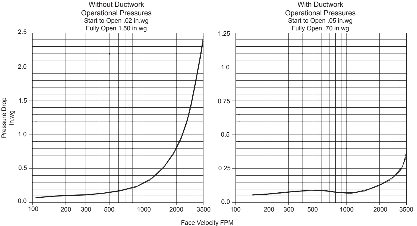
Typical performance for PRI9 backdraft damper size tested 42"W x 42"H furnished with counterweight to assist opening.
