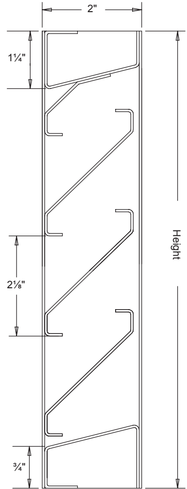
Section View
