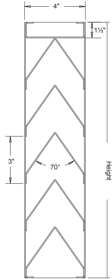
Section View
